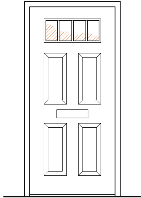
DOOR TYPE "B"
